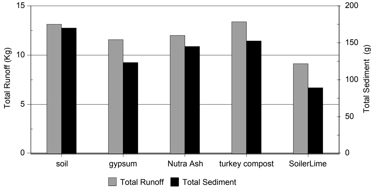
Figure 1. Total runoff and total sediment yield for each treatment.
