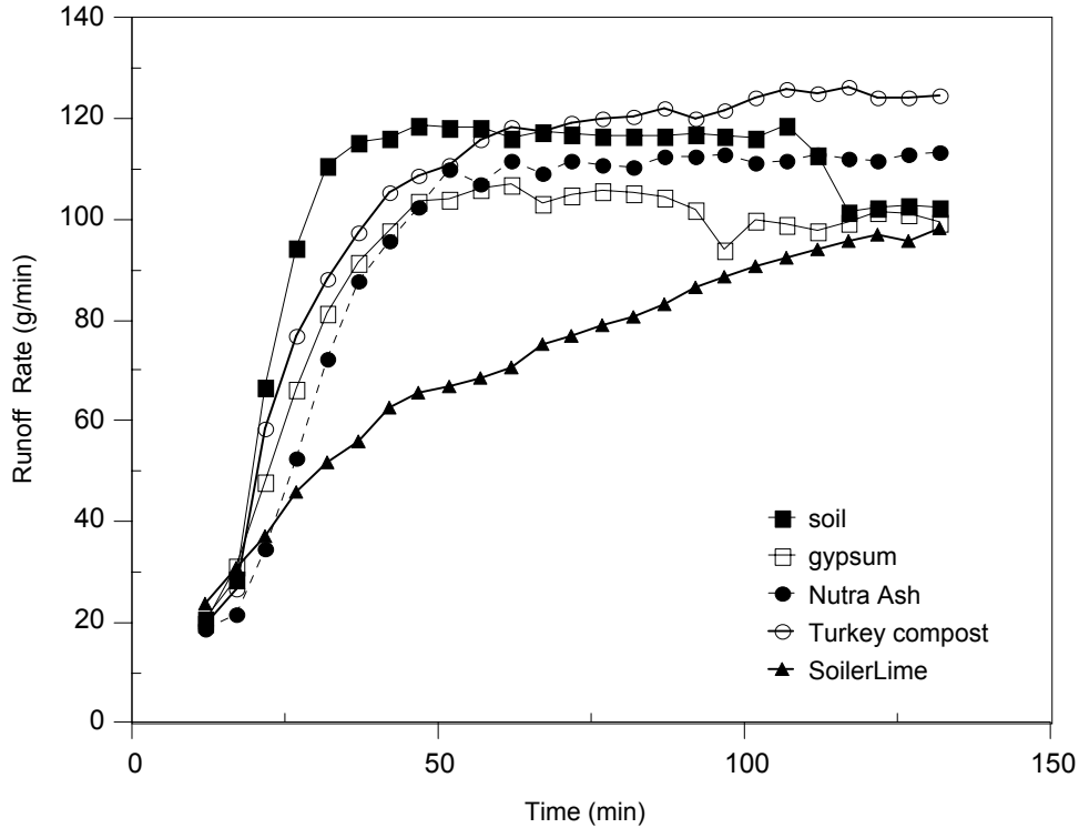
Figure 2. Runoff rate versus time for each treatment.
